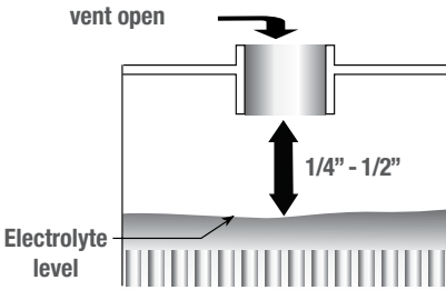
Figure 7 – Electrolyte level
