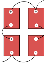
Figure 3 Voltage/Capacity Increase
