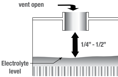
Figure 7 – Electrolyte level
